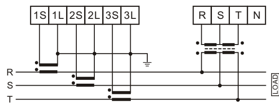
3phase 3wire (3CT. 2PT)
