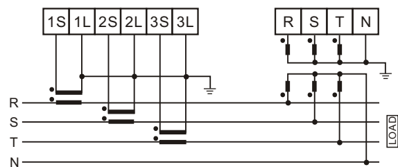
3phase 4wire
