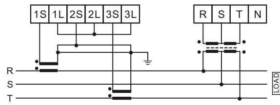
3phase 3wire (2CT. 2PT)
