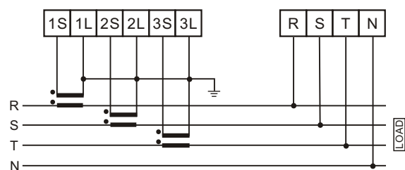
3phase 4wire (no PT)
