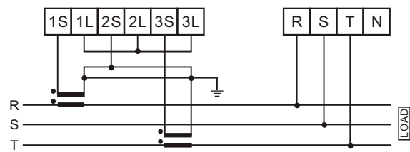
3phase 3wire (2CT. no PT)
